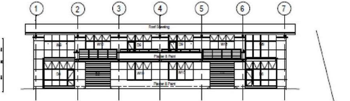
UNITS 2 & 3 WEST ELEVATION
