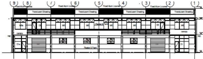
UNIT 1 NORTH ELEVATION
