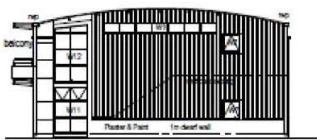
UNITS 2 & 3 SOUTH ELEVATION 1: 100
