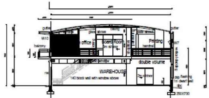
UNITS 2 & 3 SECTION B-B 1: 100
