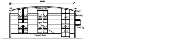
UNITS 2 & 3 NORTH ELEVATION 1: 100
