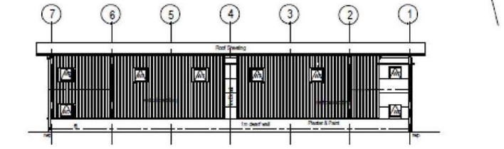
UNITS 2 & 3 EAST ELEVATION
