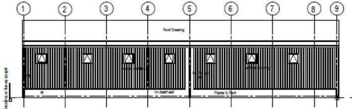
UNIT 1 SOUTH ELEVATION
