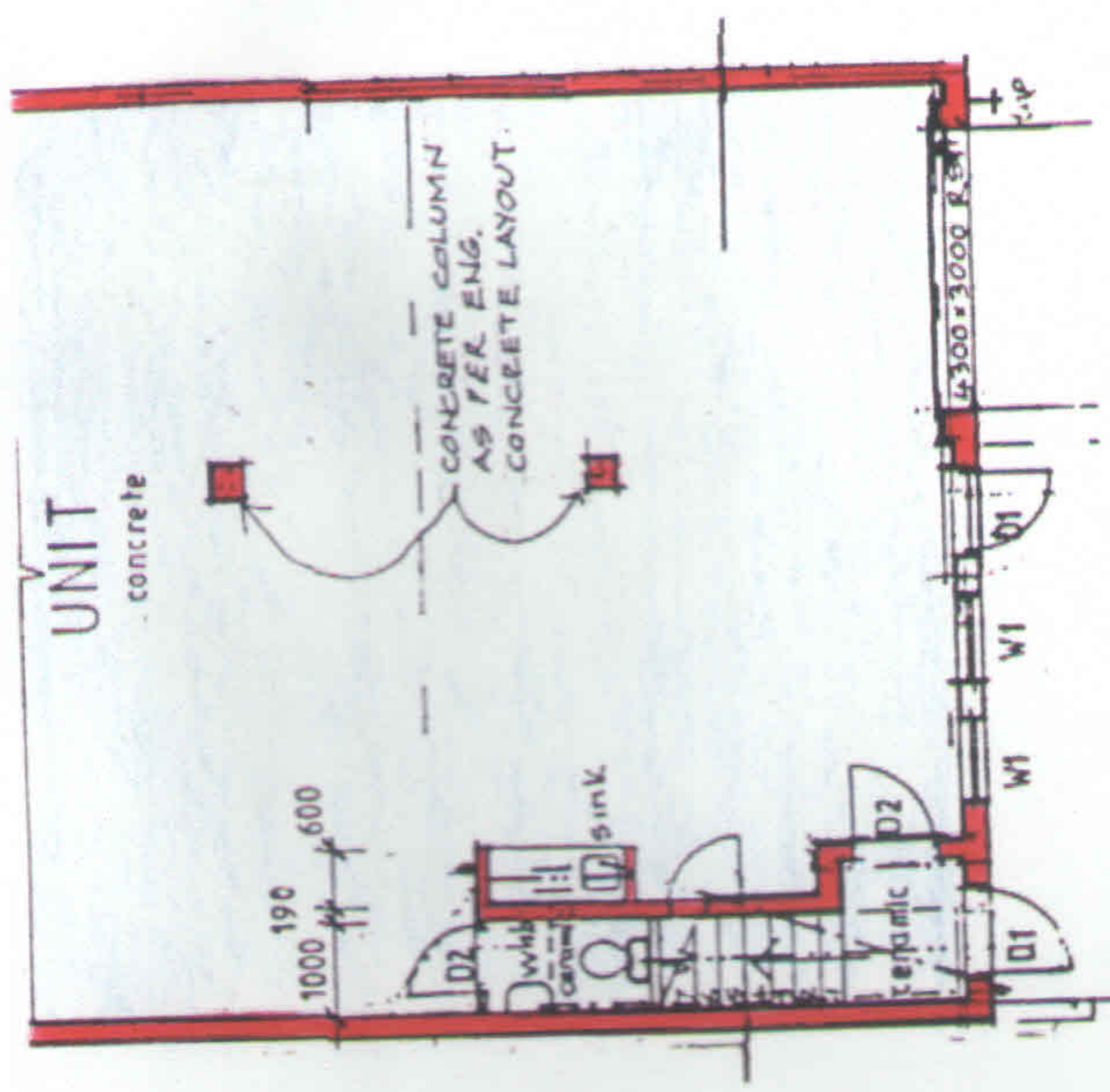
GROUND FLOOR
