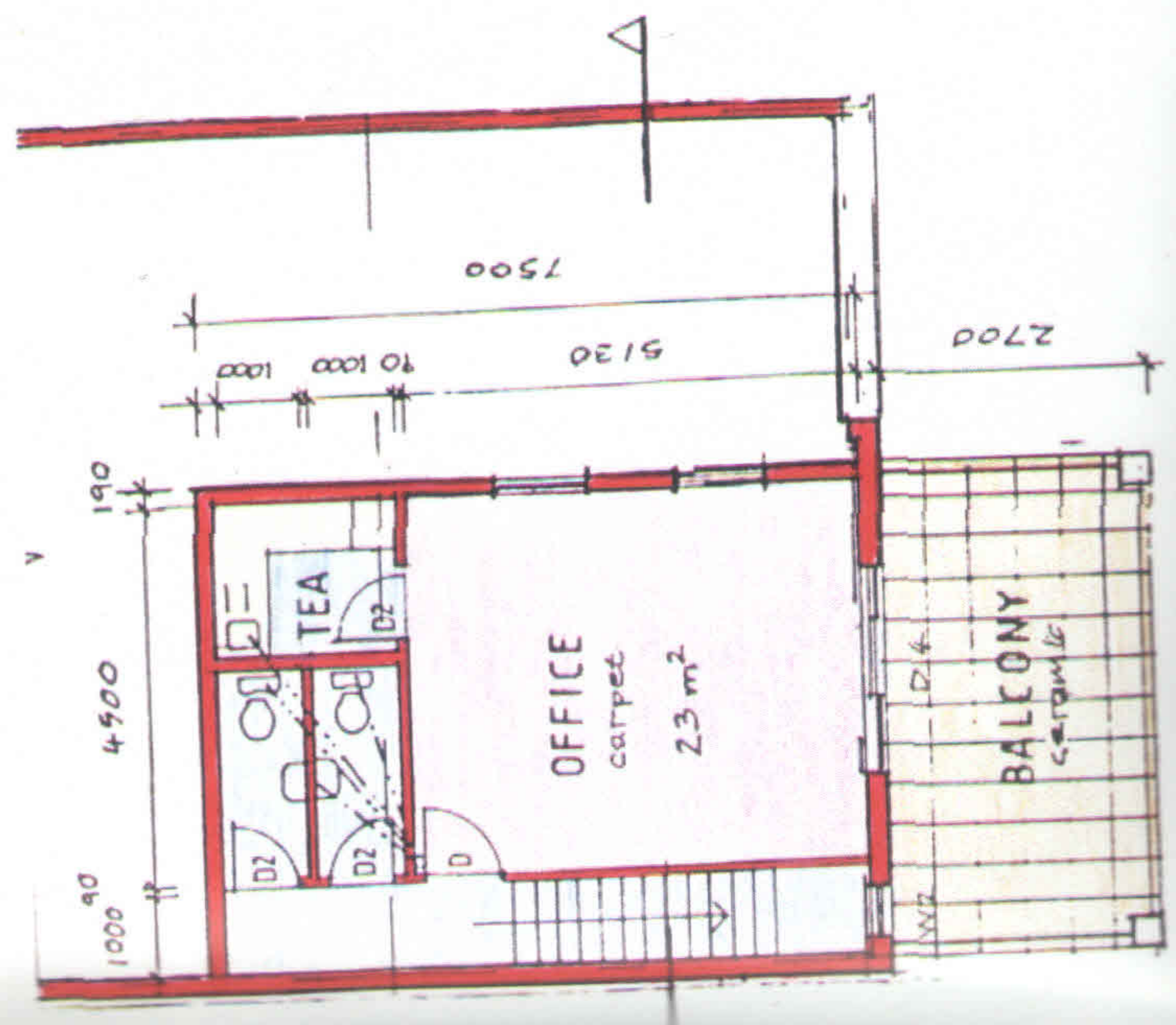
FIRST FLOOR - TYPE A: UNITS 4-11; 18-23
