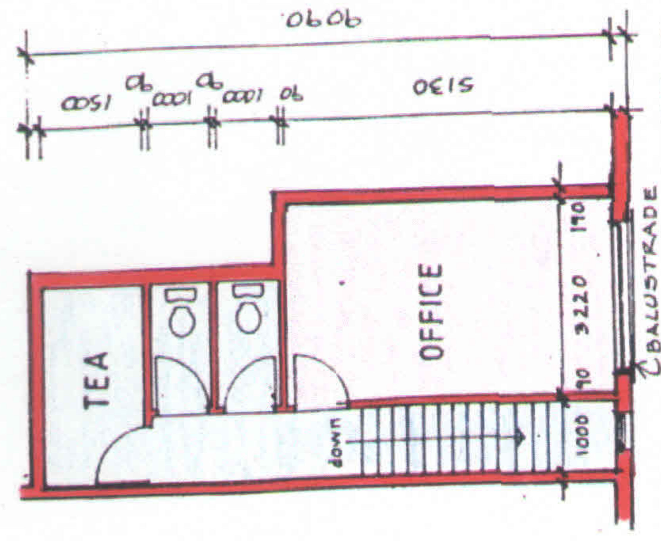
FIRST FLOOR - TYPE B: UNITS 2;3;12-16 38 m 2
